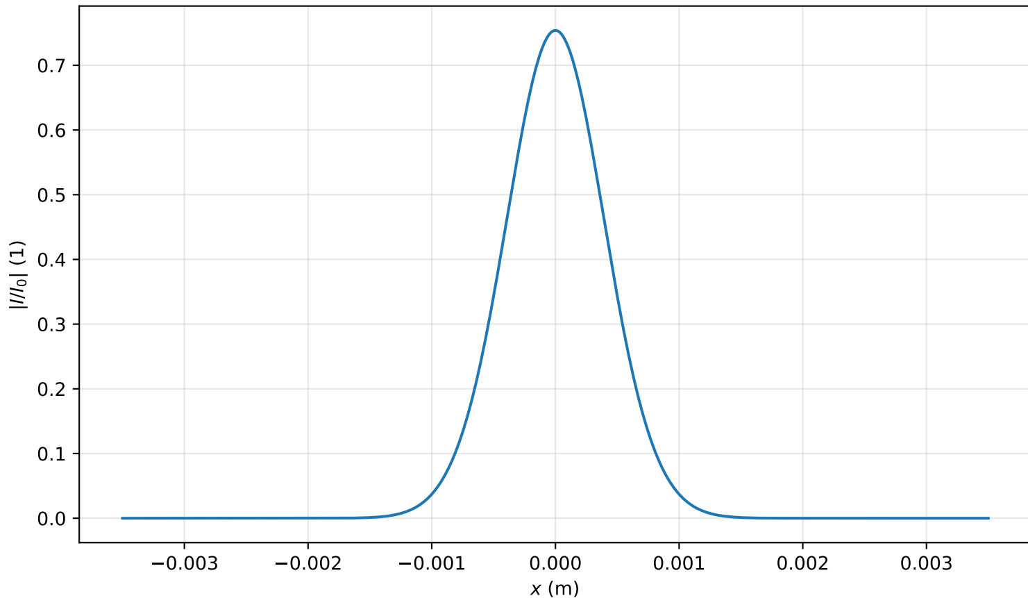
Intensity profile I(x, y = 0, z = 1.274m)/I_0 , P_{in}=0.1P_{cr} , artificial time
